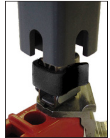
Meter socket with hot socket gap indicator testing before & after the socket safety clip is installed
