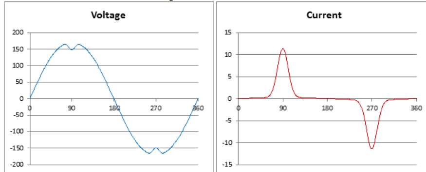
Figure 5: Pulse Waveform
