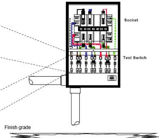
Instrument Transformer Meter Socket with Test Switch
