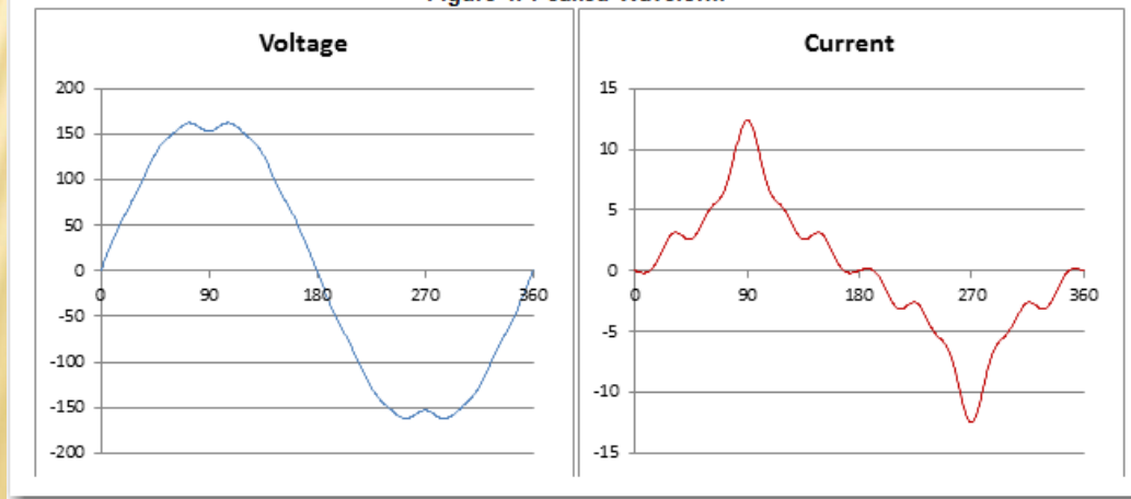
Figure 4: Peaked Waveform
