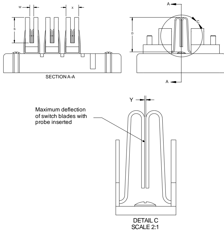
Figure 4 – Test switch typical cross section
