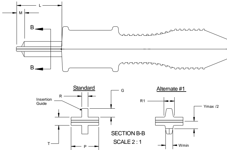
Figure 6 – Typical test plug
