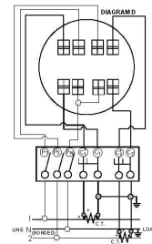
3Ø4W 'Y' with 2 P.T.'s & 3 C.T.'s 2 ½ Stator Meter - Form 6S 13T Socket
