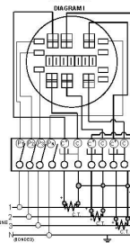
3Ø4W 'Y' or 'A' with 3 C.T.'s 'Y' 3 Stator Meter - Form 9S 'A' 2 Stator Meter - Form 6S 13T Socket
