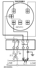
3Ø3W 'A' with 2 P.T.'s & 2 C.T.'s 2 Stator Meter - Form 5S 8T Socket
