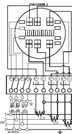
3Ø4W 'Y' with 3 P.T.'s & 3 C.T.'s 3 Stator Meter - Form 9S 13T Socket
