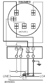
3Ø3W 'A' with 2 C.T.'s 2 Stator Meter - Form 5S 8T Socket
