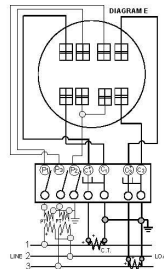
3Ø4W 'Y' or 'A' with 3 C.T.'s 'Y' 3 Stator Meter - Form 9S 'A' 2 Stator Meter - Form 6S 13T Socket
