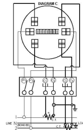
3Ø4W 'Y' with 3 C.T.'s 2 ½ Stator Meter - Form 6S 13T Socket
