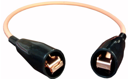
A-BASE JUMPER CATALOG NO. 202-4AWG
