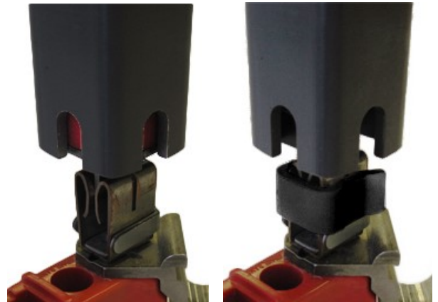
METER SOCKET WITH HOT SOCKET GAP INDICATOR TESTING BEFORE & AFTER THE SOCKET SAFETY CLIP IS INSTALLED
